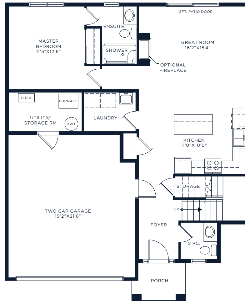
GROUND FLOOR 1,060 SQ.FT.
