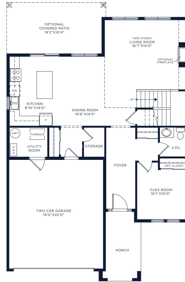
GROUND FLOOR 1,131 SQ.FT.
