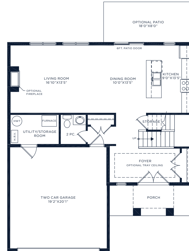
GROUND FLOOR 900 SQ.FT.
