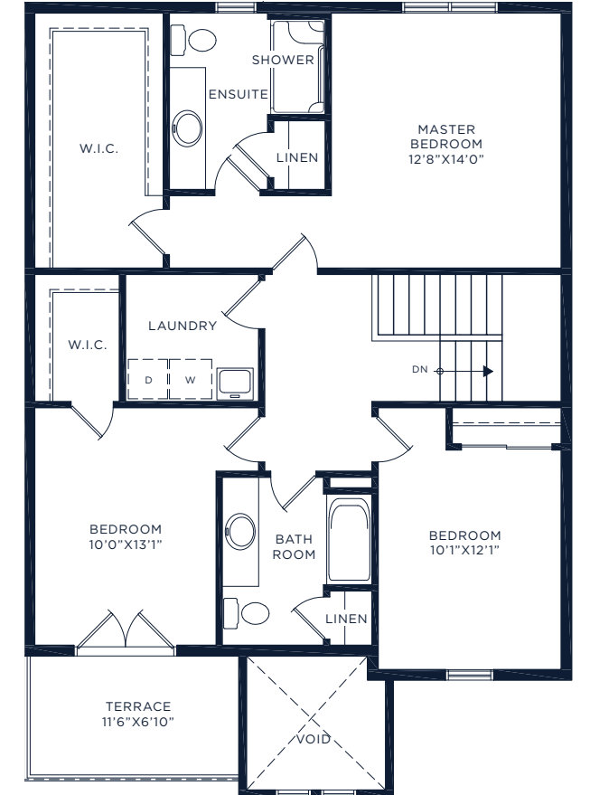
SECOND FLOOR 1,100 SQ.FT.
